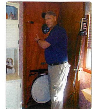
A Weatherization inspector gives a blower door demonstration on a home that has been weatherized in Howell, Mich.
